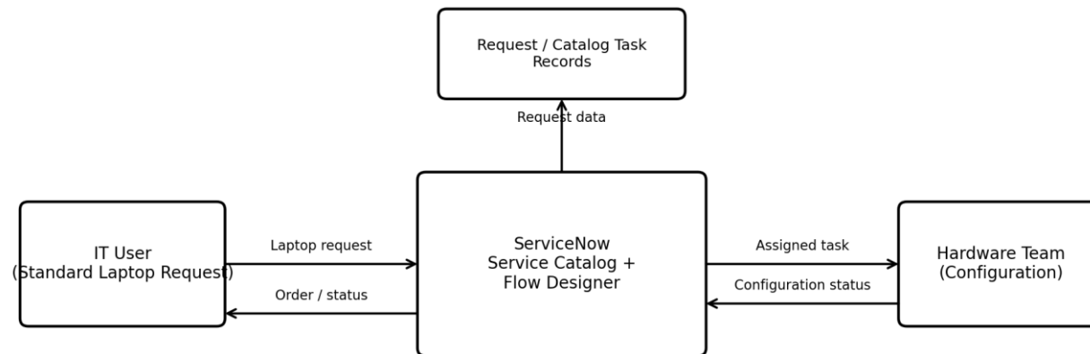
Level 0 DFD - Automated Standard Laptop Procurement
